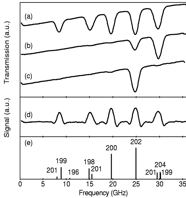
Figure 2: Ultra-violet absorption spectra from low-pressure mercury cells containing the natural isotopic mixture of atoms a) and separated isotopes b) and c). d) is a wavelength-modulated spectrum and e) the designations and relative strengths of natural mercury isotope lines.
