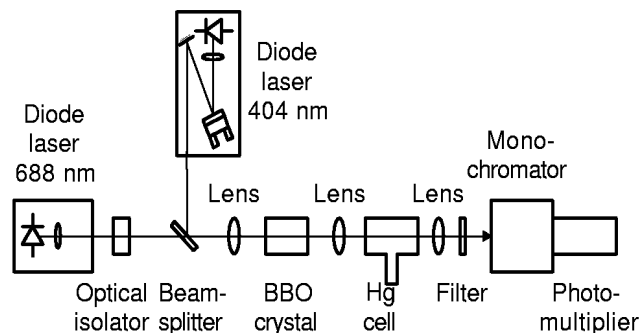
Figure 1: Experimental set up for atomic mercury monitoring using sum-frequency generation.
